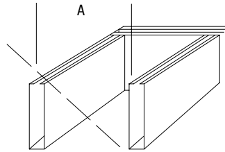
"B" Shielding Angle Open Cell blade size is 3/8" wide x 2" deep
